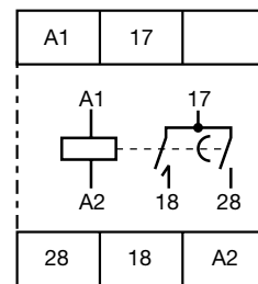
CT-SAD.22
