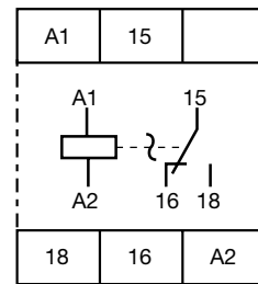
CT-EBD.12
