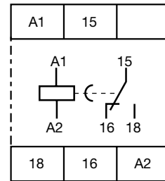
CT-ERD.12
