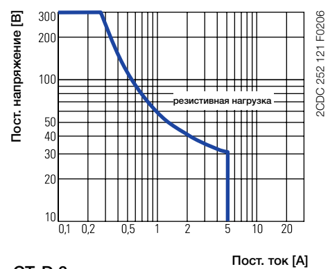
CT-D.2x
